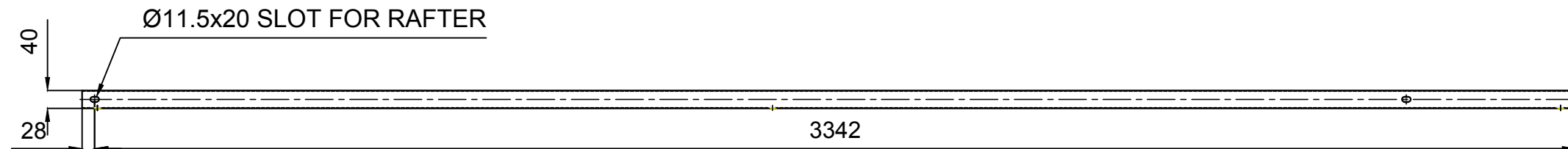
BOTTOM VIEW
