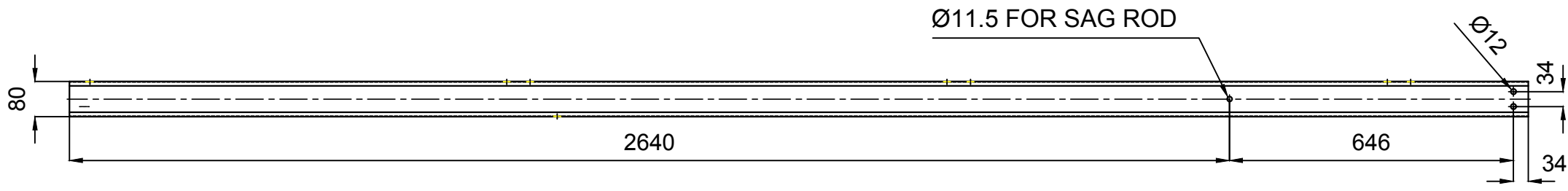
FRONT VIEW
